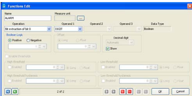
Fig.5.13. Editing functions for bit extraction.
