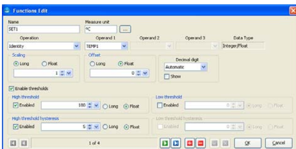
Fig. 5.7 Function edit to set an alarm on High threshold
