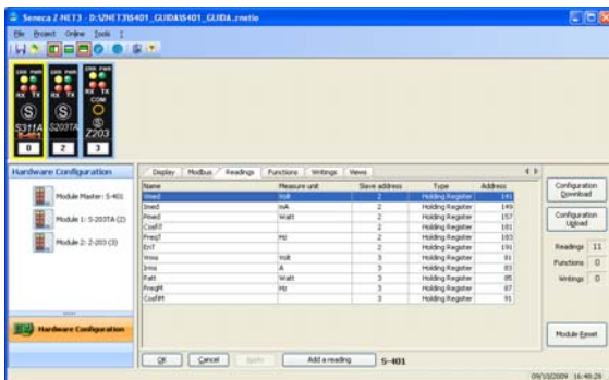
Fig. 5.2. Readings definition from S203TA and Z203
