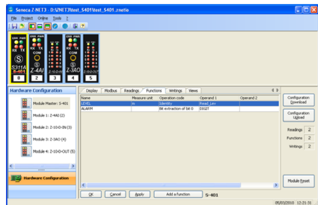
Fig.5.11 Readings definition to repeat
